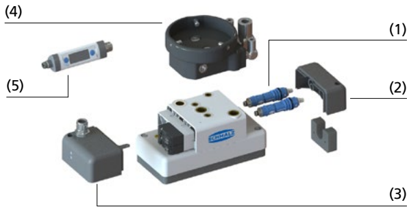
System design Area Gripping Systems FQE-X
